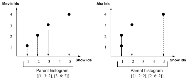
Figure 2. Node and Parent ids have a Correspondence
