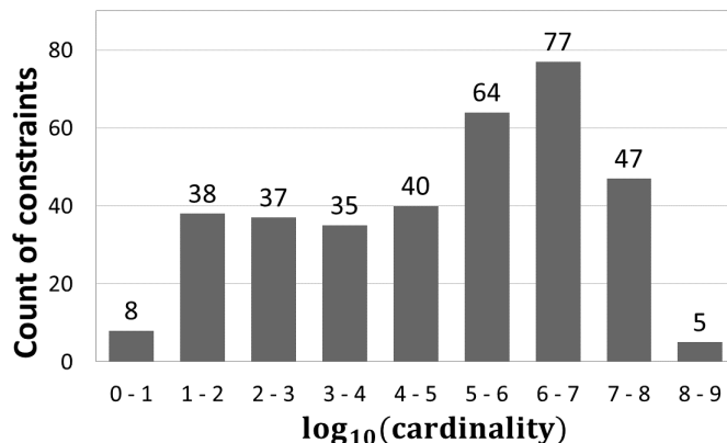
Figure 10: Distribution of Cardinality in CCs ( WL_c )
