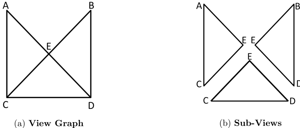
Figure 3: View Decomposition
