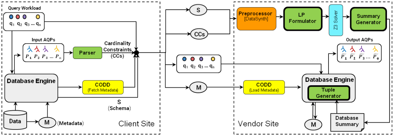
Figure 2: Hydra Architecture
