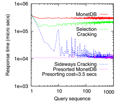
Figure 6: Skewed workload
