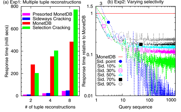
Figure 4: Improving tuple reconstruction
