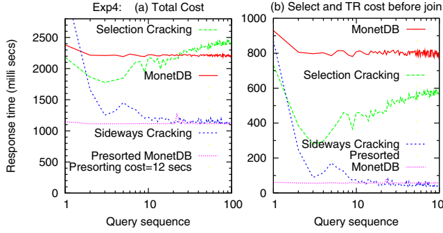
Figure 5: Join queries with multiple selections and tuple reconstructions (TR)
