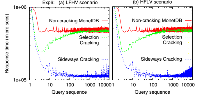
Figure 7: Effect of updates
