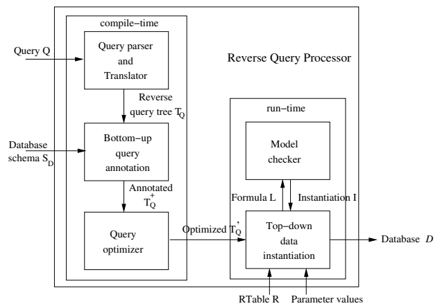
Figure 1. RQP Architecture
